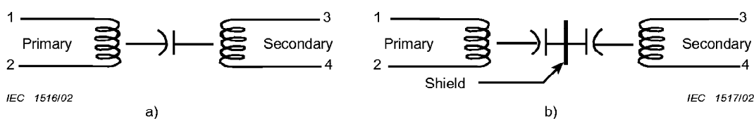
Figure 19 – Inter-winding coupling in an isolation transformer
