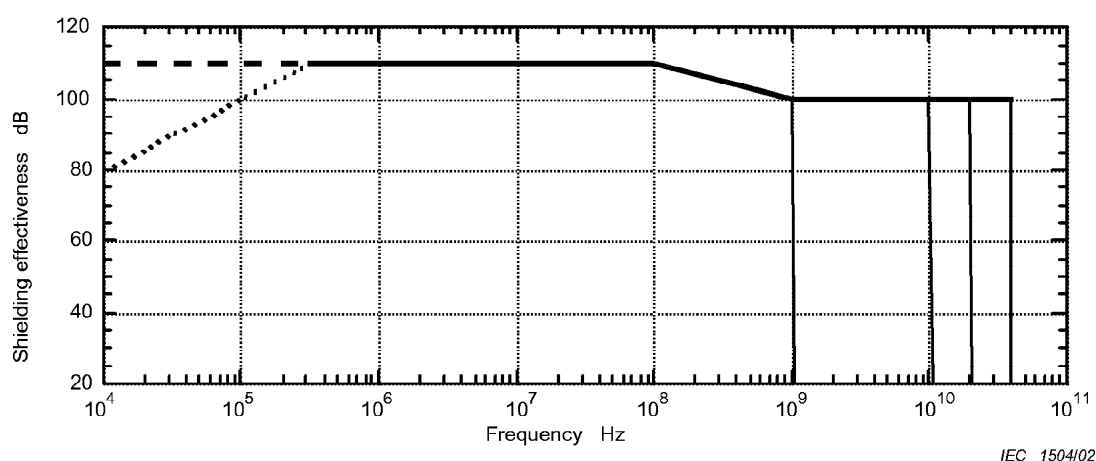
Figure 8 – Typical screening attenuation of honeycomb inserts
