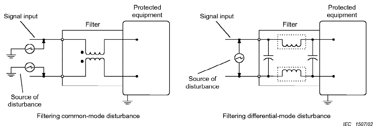
Figure 10 – Prevention of interference on installed equipment
