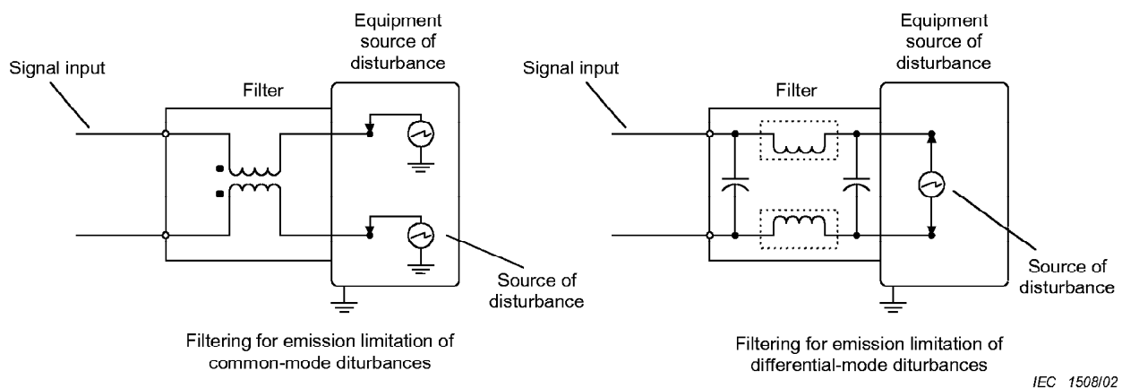
Figure 11 – Reduction of electromagnetic disturbances in the power network and the environment
