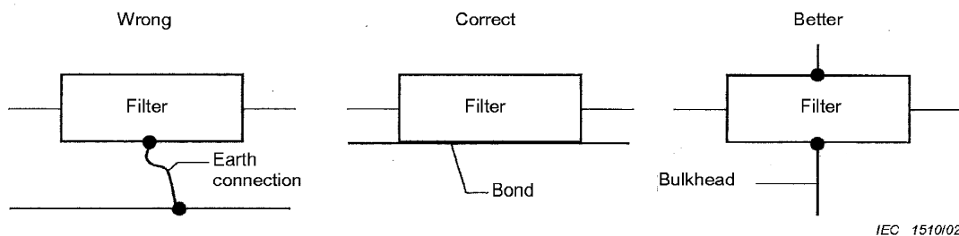
Figure 13 – Mounting of filters
