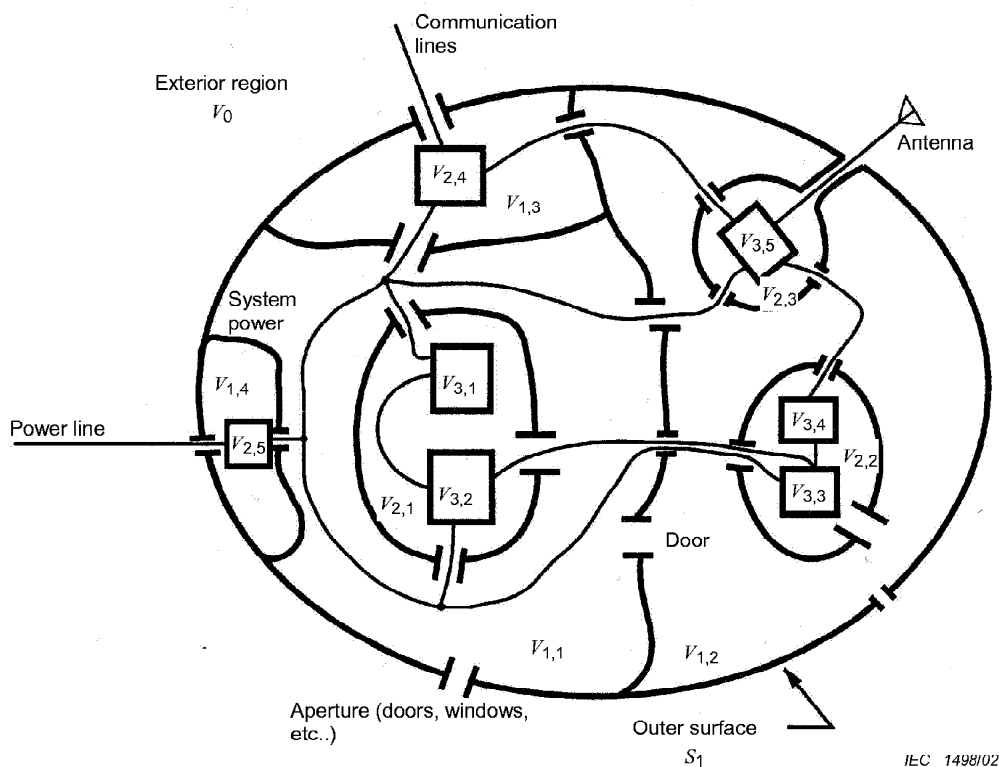
Figure 2 – Generalized system topology
