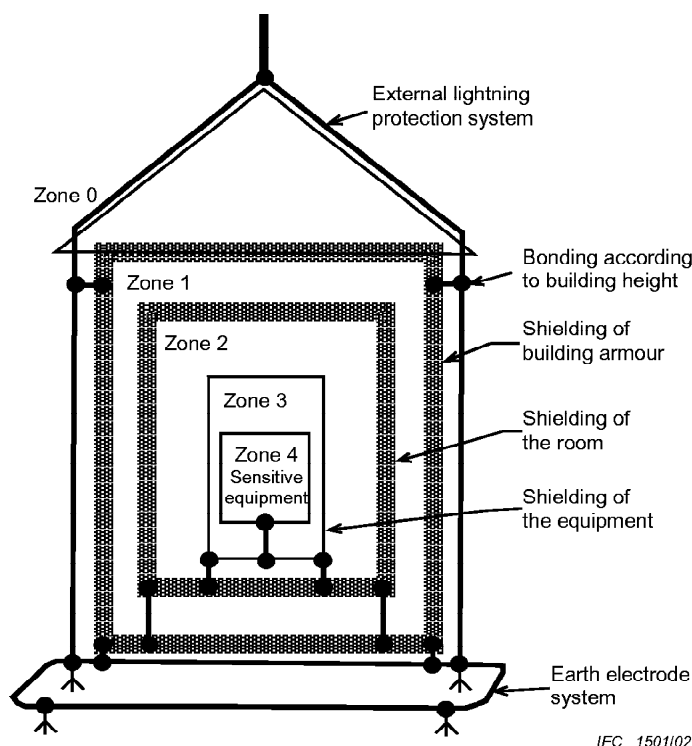
Figure 5 – Zones of protection of shielding and earthing systems
