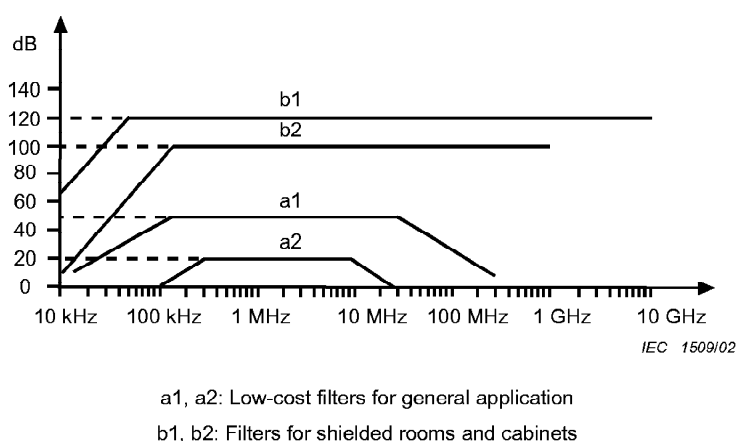
Figure 12 – Examples of insertion loss characteristics of a.c./d.c. power port filters
