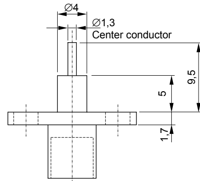
SMA-connector – Approximately 2:1
