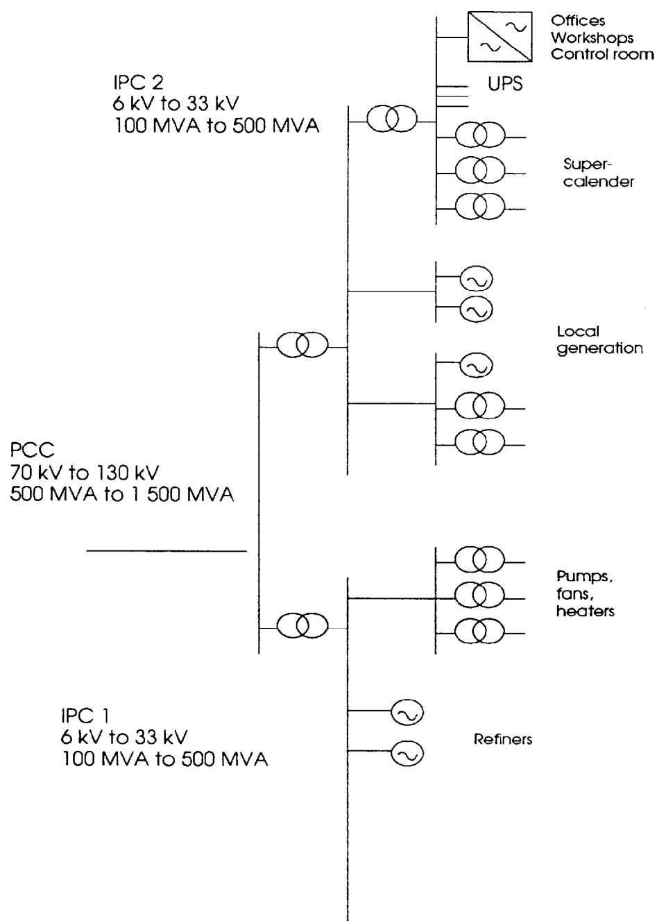
Figure A.2 – Example of power distribution in the paper industry
