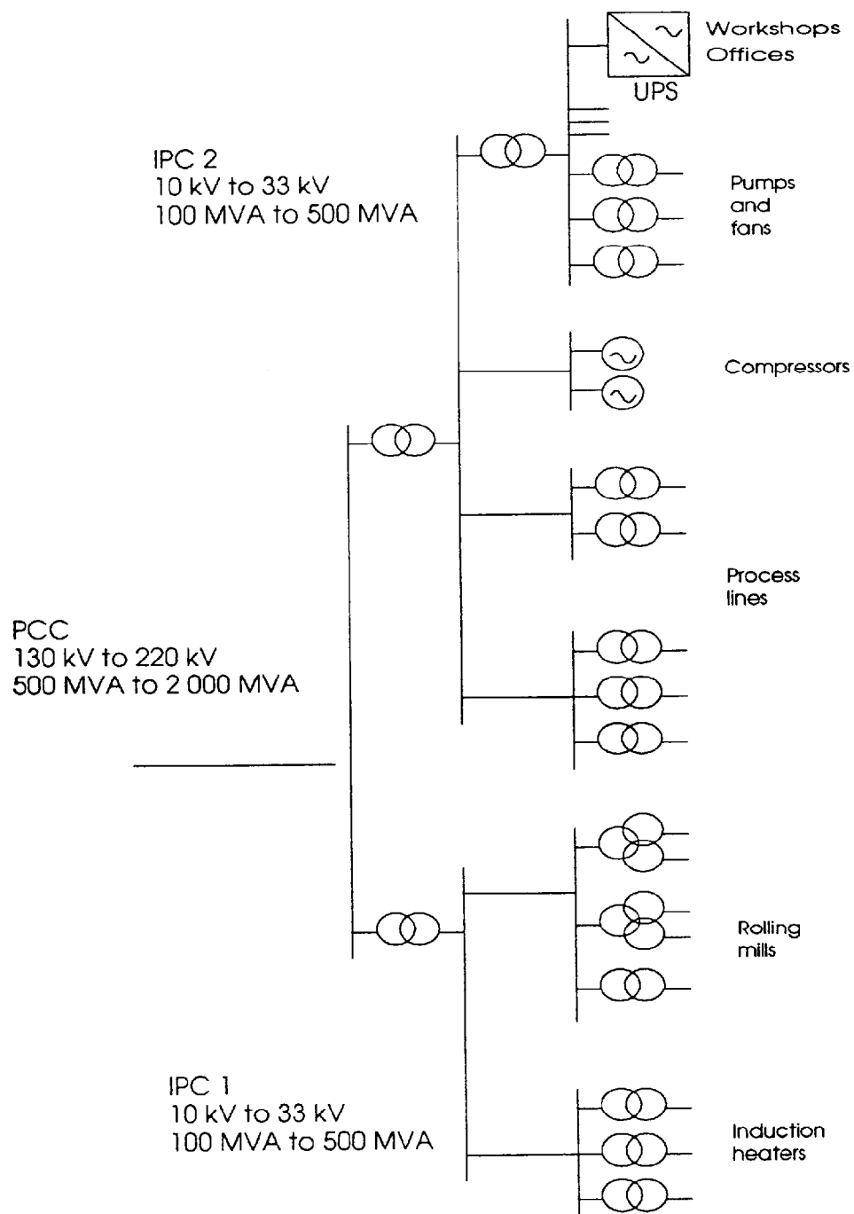
Figure A.1 – Example of power distribution in industry with rolling mills
