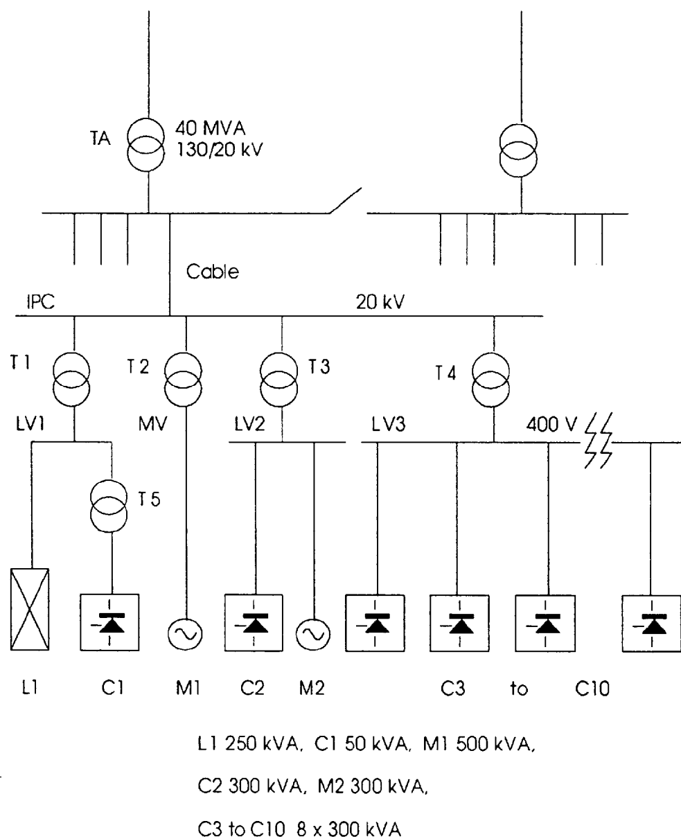
Figure A.3 – Example of power distribution in a generic manufacturing industry
